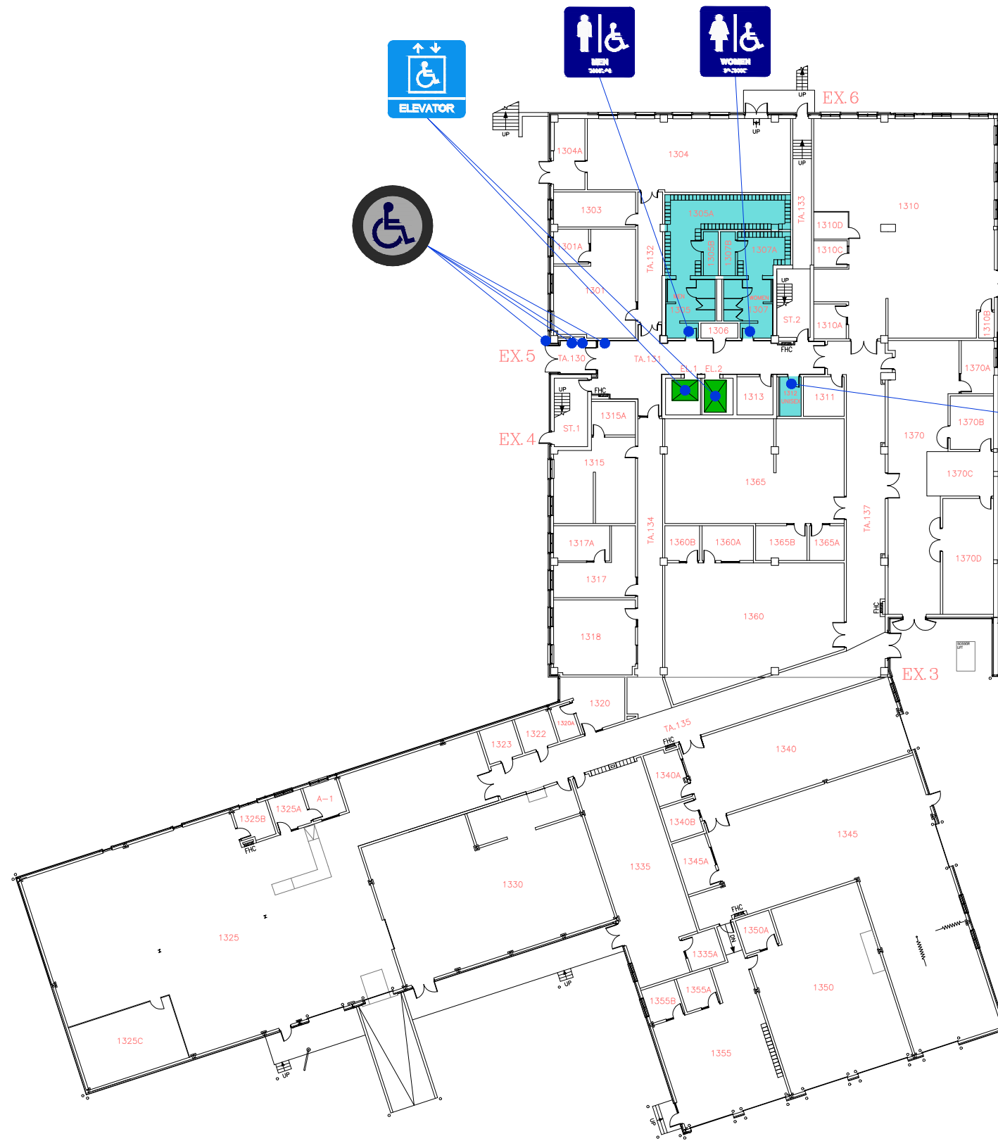
LEVEL 01 FLOOR
